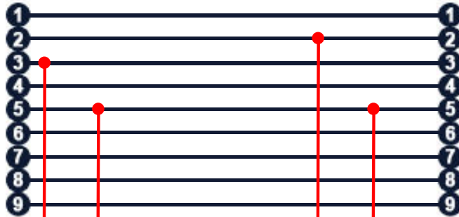
DB9 Female
